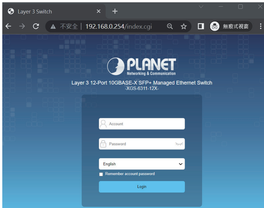
Figure 5-2: Login Screen
